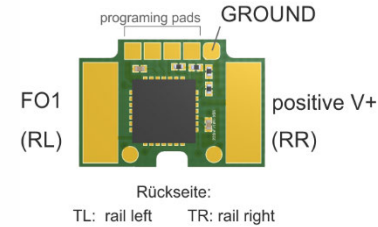
MX605FL Interior lighting function decoder
