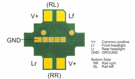
MX605SL Headlight function decoder
