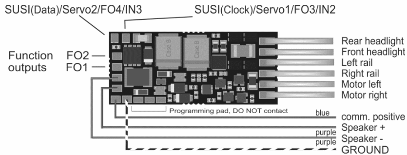
MS580N18G Bottom of the version G
