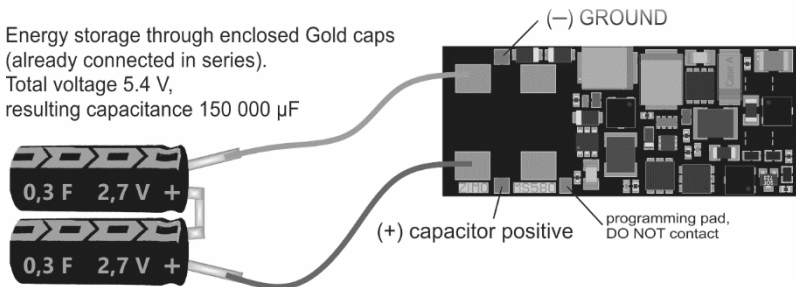
MS580N18G Bottom of the version G
