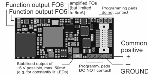
MS580N18 Top side, Next18 . SOUND
