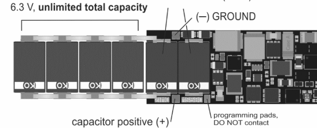
MS580N18 Bottom side, with opt. external extension of the energy storage unit
