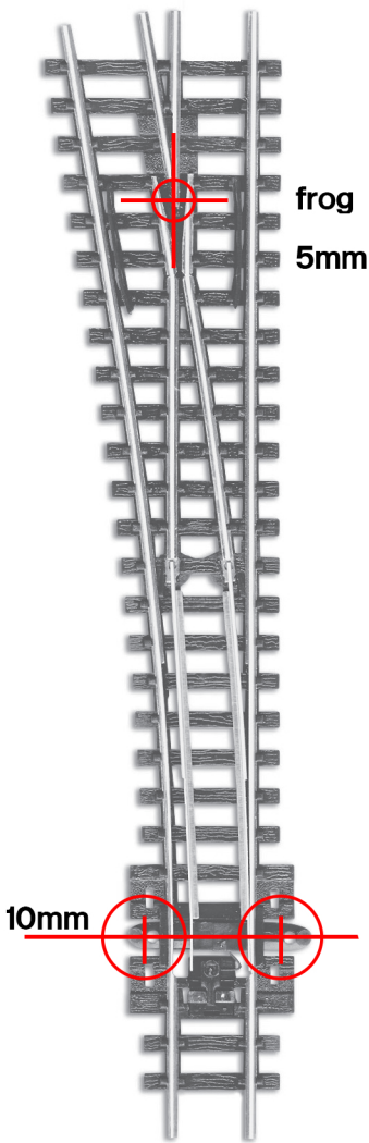
MEDIUM RADIUS TURNOUT LEFT HAND Code 55 SL-E396F Electrofrog
