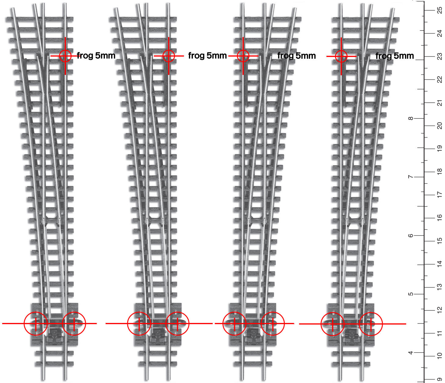
LARGE RADIUS TURNOUT LEFT HAND Code 55 SL-E389F Electrofrog
